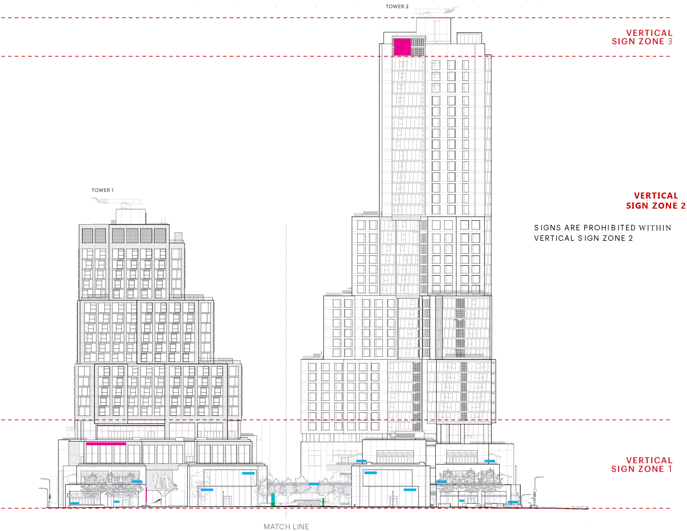
WEST ELEVATION - GRAND AVENUE
